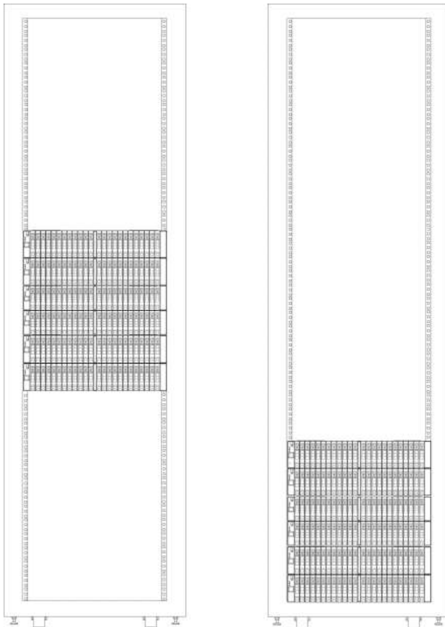
StoreServ 7400 4node Storage system in a storage centric configuration in a HP Intelligent Series Rack
